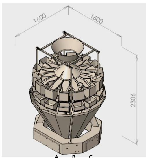
CMB14-FFW 1600 1600 2306 mm
